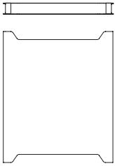
Free-standing cable management panel 1BE0194 : L 51,5 D 5 H 62
